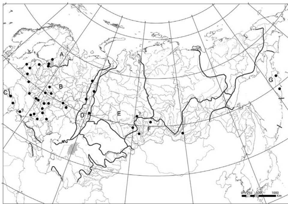
Figure 21. Localities of Arboricaria subopaca in Russia and other post-Soviet republics. Main physiological areas accepted in Mikhailov (1997, 2013) are indicated: A Fennoscandia B Russian Plain C Carpathians D Urals E West Siberia F mountains of South Siberia G Kamchatka.
